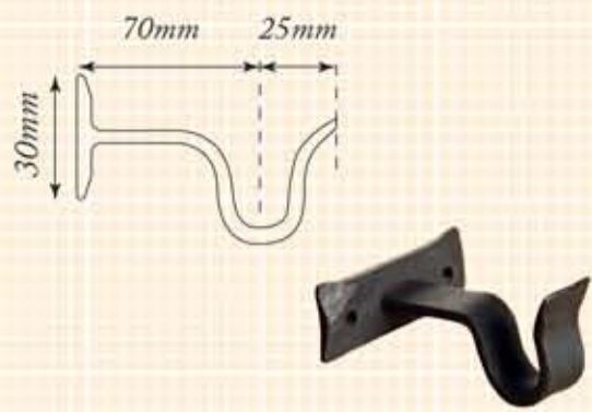
Centre bracket
